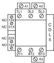
AE50 ... AE75-30-11 TAE50/75-30-11
