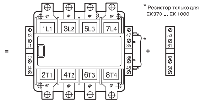
= EK110 ... EK1000-40-21 + CAL16-11C
