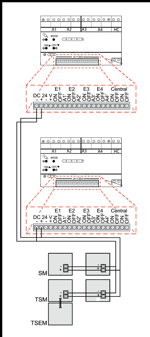
Wiring example of two Universal Dimming Stations with two sensor modules, a push-button module and a push-button module with extension unit. Simply connected via two wires.
