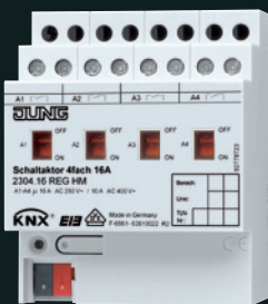
Switch actuator with C-load, 4-gang with current detection
